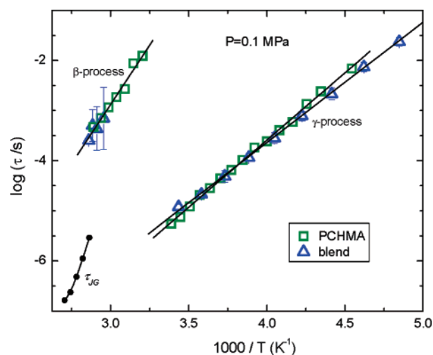
Figure 5. Relaxation times for secondary relaxations in PCHMA neat and in a 50/50 blend with PaMS. The lines are fits yielding the activation energies listed in Table 2. Also shown are the coupling model predictions for the JG relaxation times, from the experimental values of \tau_\alpha and \beta_{\text{KWW}} , with t_c = 2 \text{ ps} .
